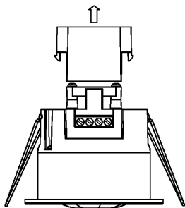
1. Removig the vinal cover.
