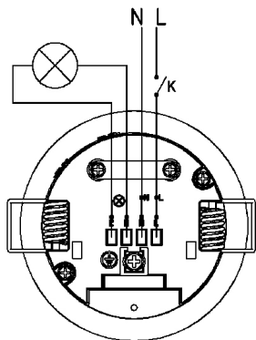
3. Wiring the motion sensor.
