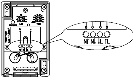
5. Wiring the twilight switch.
